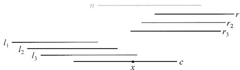
Figure 9 Detection of chimeric reads. Reads l_1, l_2, l_3, r_1, r_2, and r_3 , and the absence of a read n (having long overlaps on both sides of a point x ) suggest that read c may be chimeric, consisting of the juxtaposition of two disparate genomic segments: one corresponding to the part of c before x , and one corresponding to the part of c after x . We call x the point of chimerism of c . Note that reads l_3 and r_3 extend slightly beyond x , as often happens for real chimeric reads.
