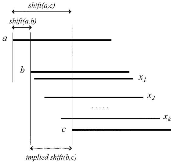
Figure 10 Contig assembly. If (a,b) and (a,c) overlap, then (b,c) are expected to overlap. Moreover, one can calculate that shift(b,c) \approx shift(a,c) - shift(a,b) . We detect a repeat boundary toward the right of read a , if there is no overlap (b,c) , nor any path of reads x_1, \dots, x_k such that (b,x_1), (x_1,x_2), \dots, (x_k,c) are all overlaps, and shift(b,x_1) + \dots + shift(x_k,c) \approx shift(a,c) - shift(a,b) .
