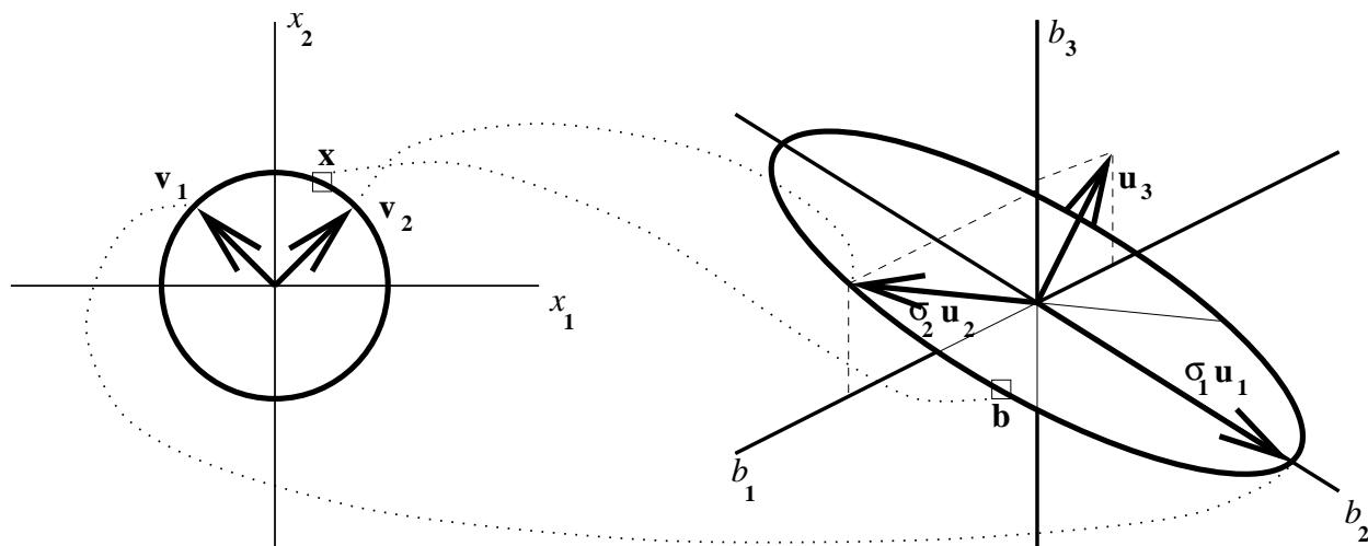
Figure 1: The matrix in equation (5) maps a circle on the plane into an ellipse in space. The two small boxes are corresponding points.
