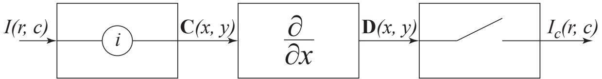
Figure 1: Conceptual bloc diagram for the computation of the derivative of image I(r, c) in the horizontal ( c ) direction. The first block interpolates from a discrete to a continuous domain. The second computes the partial derivative in the horizontal ( x ) direction. The third block samples from a continuous domain back to a discrete one.
