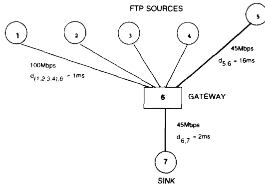
Fig. 11. A simulation network with five FTP connections.
