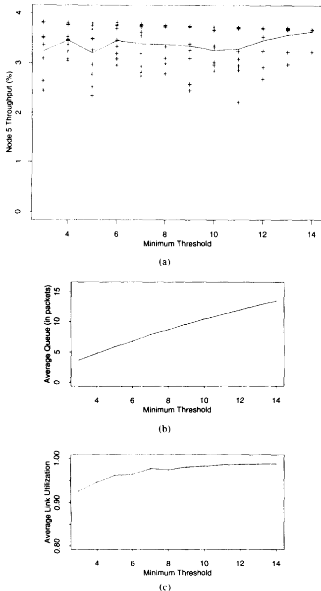
Fig. 14. Simulations with RED gateways
