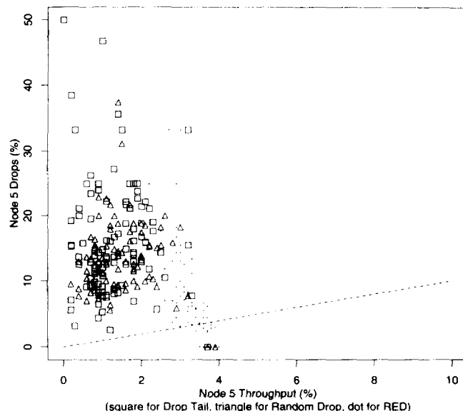
Fig. 15. Scatter plot, packet drops versus throughput.
