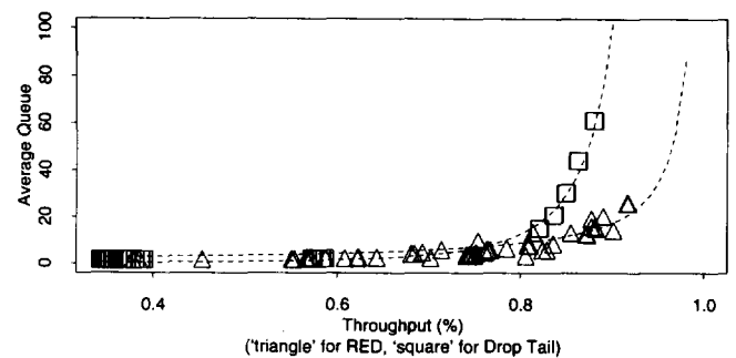
Fig. 5. Comparing Drop Tail and RED gateways.
