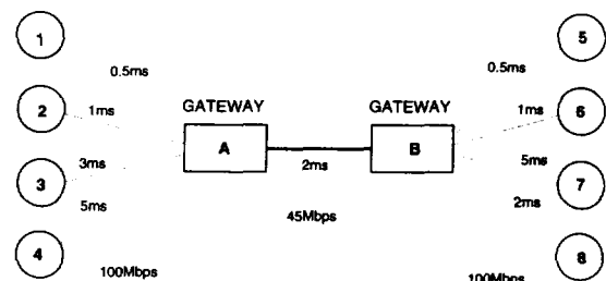
Fig. 10. A network with many short connections.
