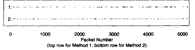
Fig. 8. Randomly marked packets comparing two packet-marking methods.
