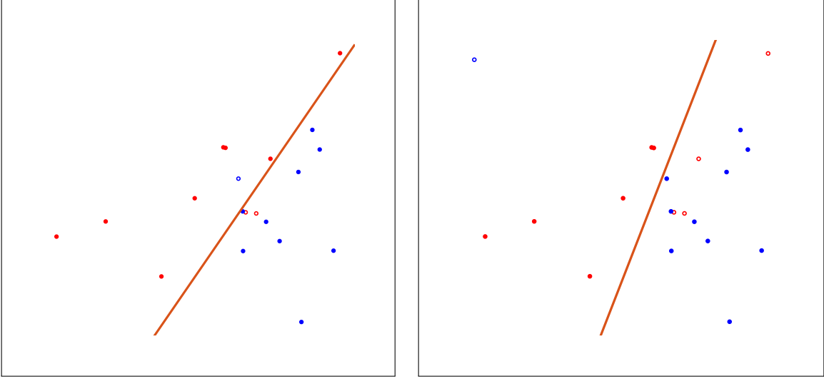
Figure 1: The color of dots in these two diagrams denotes true class membership, and hollow dots are samples that the logistic-regression classifier (whose decision boundary is the red line) misclassifies. The training sets in the two diagrams are identical, except for a single data sample added to the one on the right, close to the top-left corner. This distant sample is enough to shift the decision boundary quite a bit.
