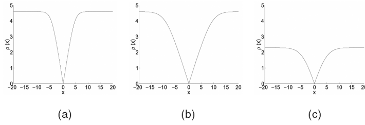
Fig. 2. (a) e = 0.01, \sigma = 1.0 . (b) e = 0.01, \sigma = 2.0 . (c) e = 0.1, \sigma = 2.0 . Robust function \rho(x) = -\ln((1 - e) \exp(-\frac{|x|}{\sigma}) + e) derived from TV model. Parameters \sigma and e , respectively, control the sharpness and the upper-bound of the function.
