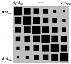
Fig. 4. Compatibility matrix \psi_{st}(x_s, x_t) . The range of disparity is [d_{min}, d_{max}] . A larger box represents a bigger value.
