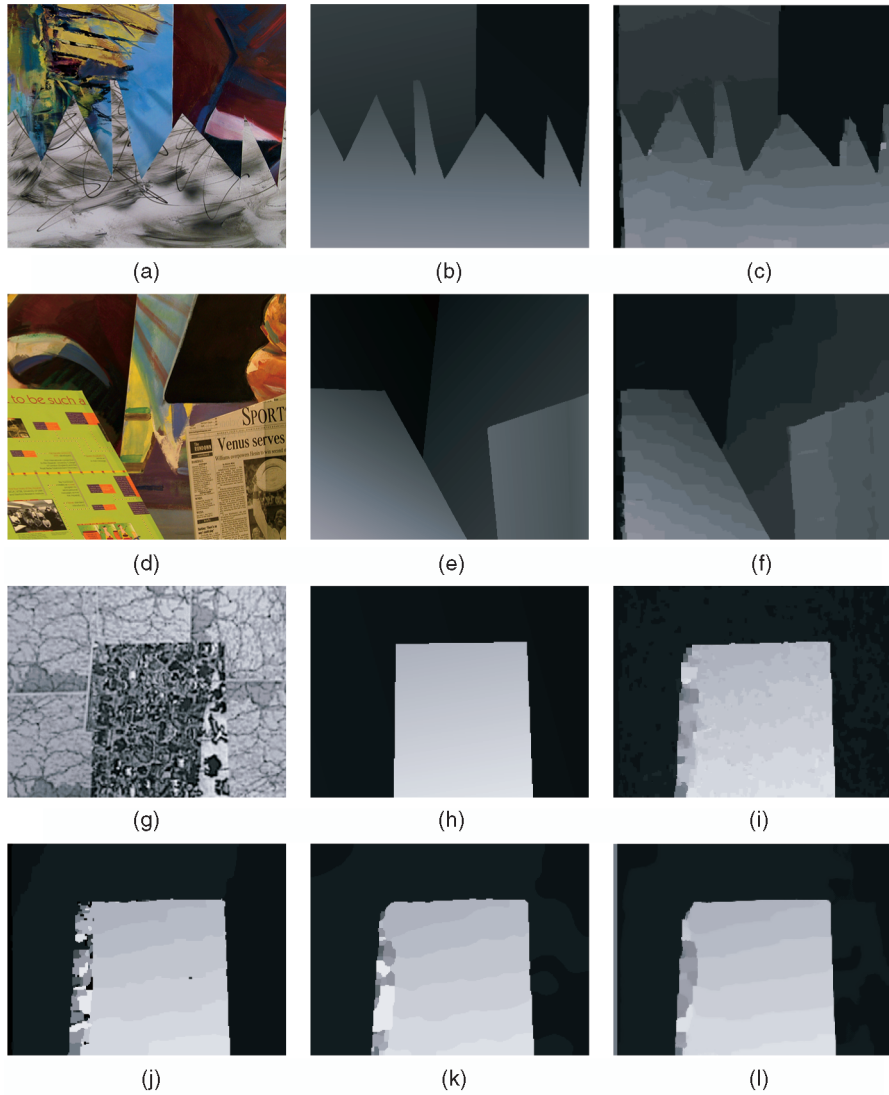
Fig. 7. (a) Sawtooth: image. (b) Ground truth. (c) Max-product result. (d) Venus: image. (e) Ground truth. (f) Max-product result. (g) Map: image. (h) Ground truth. (i) Max-product result. (j) Graph cut result. (k) Bayes diffusion result. (l) Sum-product result. The results of Sawtooth, Venus, and Map based on the “max-product” algorithm are shown in (c), (f), and (i). Graph Cut ( B_{\bar{O}} = 0.31 , B_D = 3.88 ) and Bayesian diffusion results ( B_{\bar{O}} = 0.20 , B_D = 2.49 ) are shown in (j) and (k), while the “sum-product” result ( B_{\bar{O}} = 0.16 , B_D = 2.11 ) is shown in (l).
