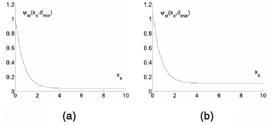
Fig. 5. (a) seg(s) = seg(t) . The left shows the first row of \psi_{st}(x_s, x_t) when node x_s and x_t are in the same region. (b) seg(s) \neq seg(t) . The right shows the first row of \psi_{st}(x_s, x_t) when node x_s and x_t are in different regions. ( \{\epsilon_p = 0.01, \sigma_p = 1.0, \lambda_{seg} = 0.05\} ).
