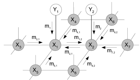
Fig. 3. Local message passing in a Markov Network. Gray nodes are hidden variables. White nodes are observable variables. In the "max-product" algorithm, the new message sent from node x_1 to x_2 is: m_{1,2}^{new} \leftarrow \kappa \max_{x_1} \psi_{12}(x_1, x_2) m_{1,3} m_{3,1} m_{4,1} m_{5,1} . The belief at node x_1 is computed as: b_1 \leftarrow \kappa m_{1,2} m_{2,1} m_{3,1} m_{4,1} m_{5,1} .
