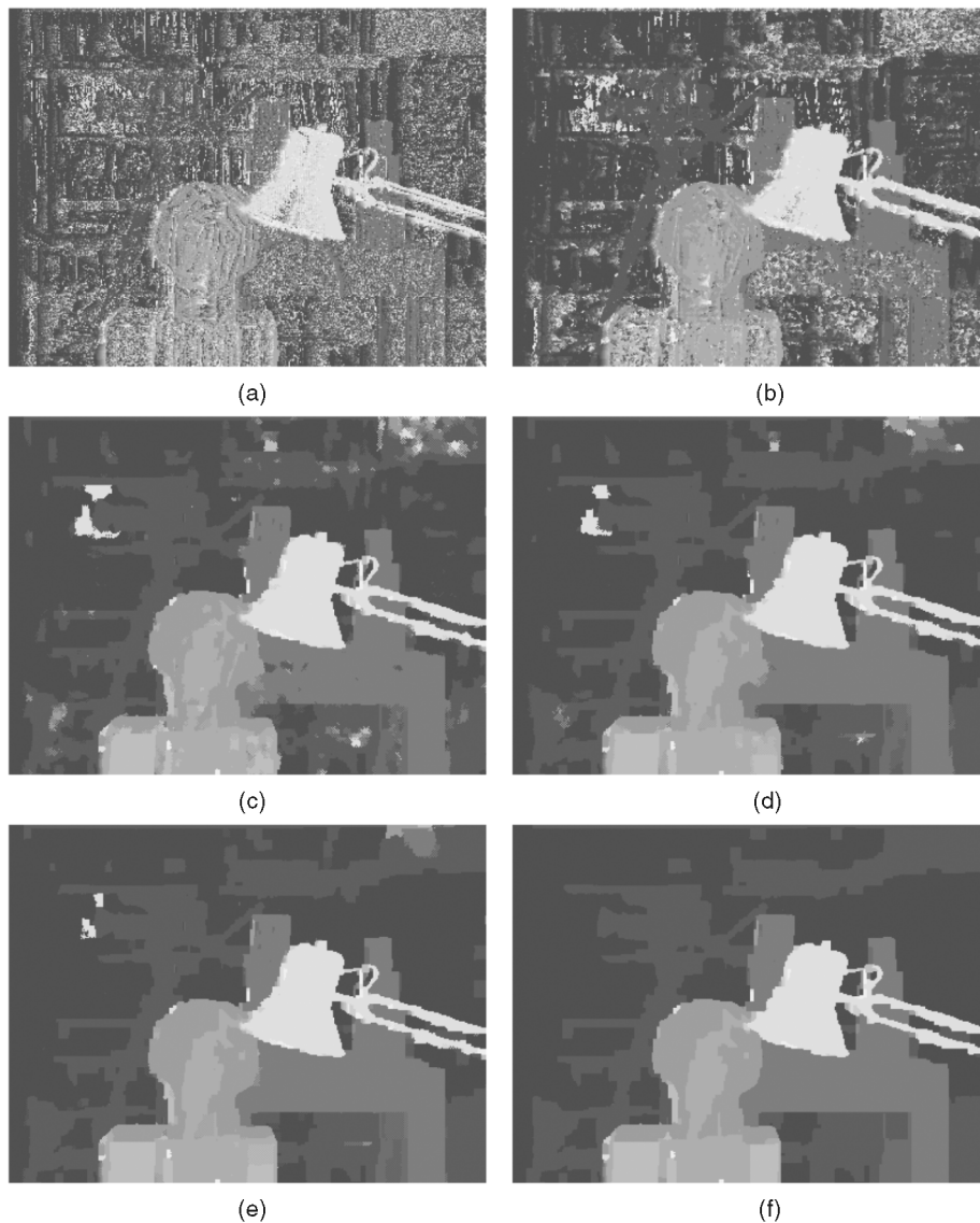
Fig. 8. (a) Iteration (0). (b) Iteration (1). (c) Iteration (8). (d) Iteration (16). (e) Iteration (32). (f) Iteration (64). Intermediate results on Tsukuba data at different iterations.
