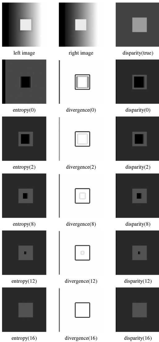
Fig. 14. Time-varying adaptive smoothing mechanism of the BP algorithm in stereo matching is illustrated from row 2 to row 6. The input image pair and the ground truth are shown in the first row. The number of the iterations is shown in the parentheses.
