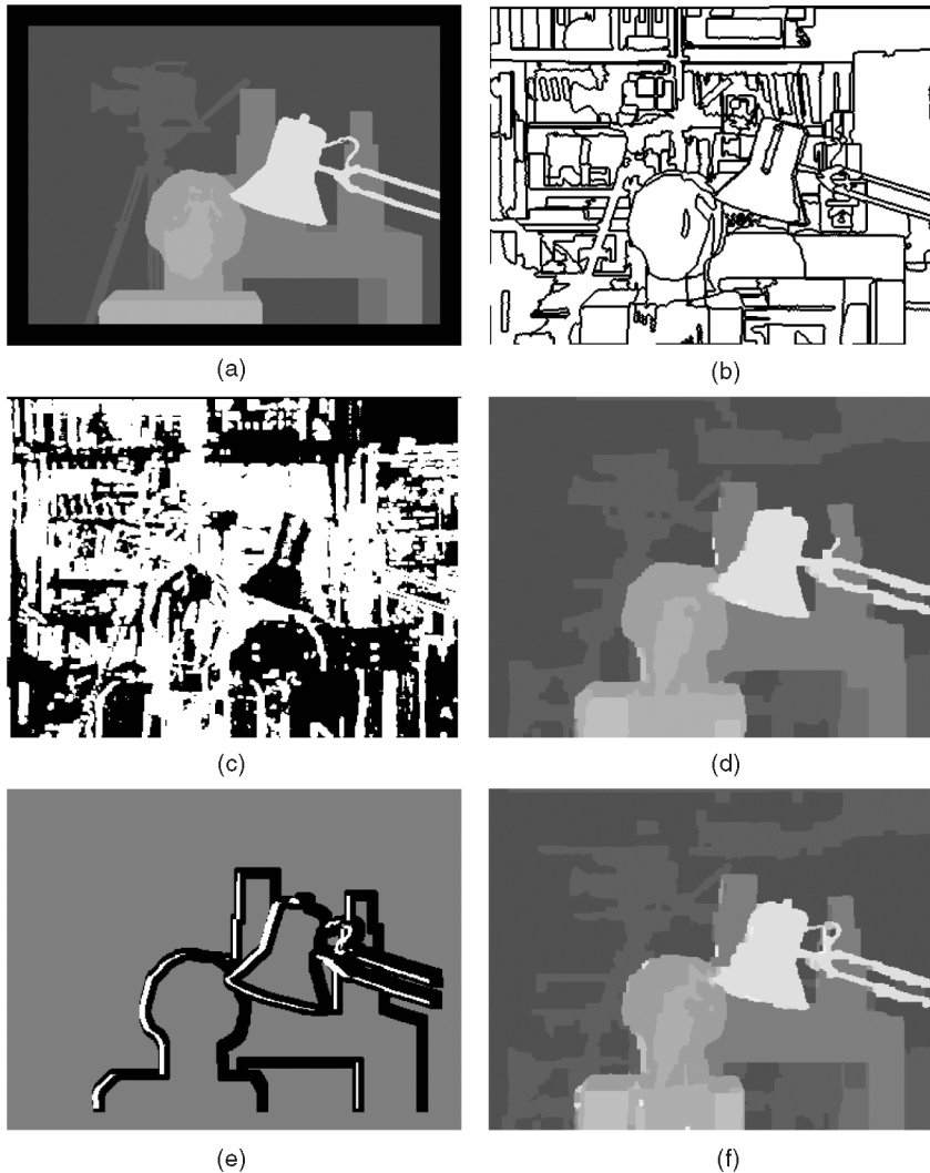
Fig. 6. The results on the Tsukuba data set. (a) Ground truth. (b) Image segmentation result. (c) Textureless regions. (d) Max-product result without segmentation. (e) Discontinuity (white) and occlusion (black) regions. (f) Max-product result with segmentation.
