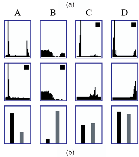
Fig. 9. Local evidence with different convolution kernels. (a) Four points (A, B, C, and D) in the sixth frame of the “garden” sequence (11 frames) are semiocclusion points. (b) Each column corresponds A, B, C, and D, respectively. The first row shows local evidence \Psi_s(x_s, y_s) using convolution kernel w_d(s, d_s, k) . The horizontal and vertical coordinates are disparity and matching probabilities, respectively. The second row shows local evidence \Psi_s(x_s, y_s) using convolution kernel w_f(s, d_s, k) . The last row shows F^- (black) and F^+ (gray). The evidences marked with a black rectangle at the top right corner are computed by our convolution kernel w_a(s, d_s, k) .
