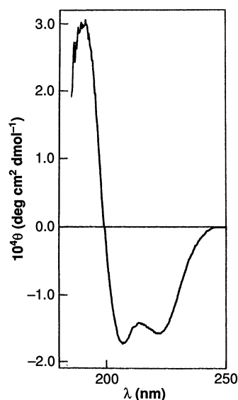
Fig. 9. Circular dichroism spectrum of Felix S-S. Felix S-S was dissolved at 0.09 mg/ml (~10 μM) in 50 mM sodium phosphate, pH 7.6 in a cuvette with a 1-mm path length. Spectra were measured at 2°C with a Jobin Yvon Mark 5 spectropolarimeter interfaced with an Apple computer. The data were collected in triplicate from 260 nm to 185 nm with a step size of 0.2 nm, and a response time of 2 seconds.
