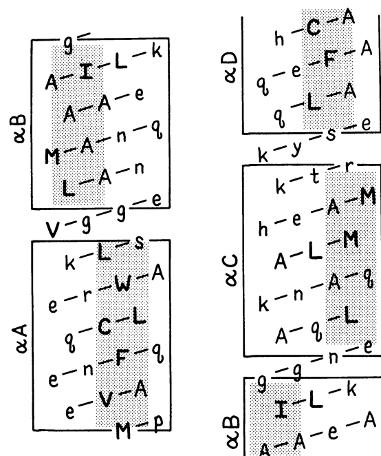
Fig. 3. A helical net with 3.5-residue pitch, continuous through the helices of Felix. The hydrophobic stripe on each helix is indicated, showing how they are offset across the designed helix connection to prevent formation of a single coiled-coil helix.
