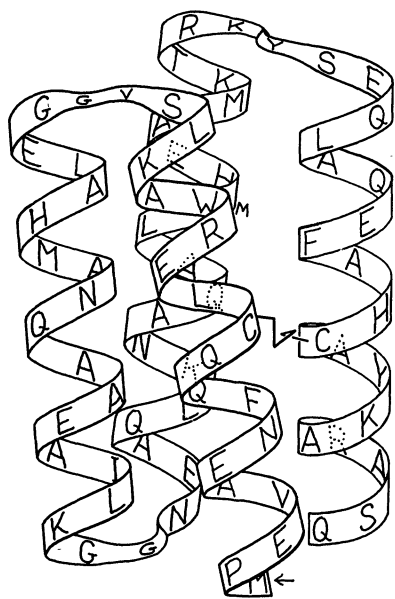
Fig. 1. Ribbon drawing of the sequence and proposed three-dimensional structure of Felix, with the disulfide indicated. The chain turns left at the top of the first helix, making this a "left-turning", up-and-down, four-helix bundle. Abbreviations for the amino acid residues are: A, Ala; C, Cys; D, Asp; E, Glu; F, Phe; G, Gly; H, His; I, Ile; K, Lys; L, Leu; M, Met; N, Asn; P, Pro; Q, Gln; R, Arg; S, Ser; T, Thr; V, Val; W, Trp; and Y, Tyr.
