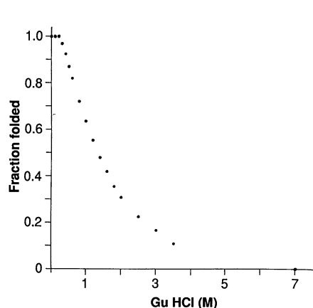
Fig. 10. Denaturation of Felix S-S. The fraction of protein in the native state (calculated as the ratio between the observed mean residue ellipticity at 222 nm at a given concentration of denaturant relative to the observed value in the absence of denaturant) versus the concentration of Gu-HCl. The procedures were as described for Fig. 9, except that the denaturation was performed at 20°C.
