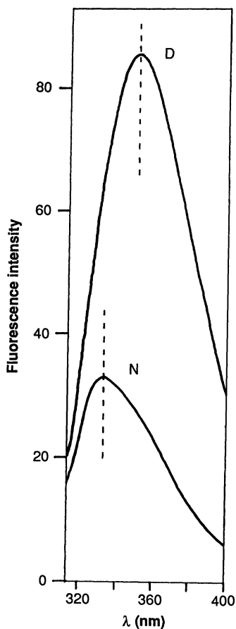
Fig. 11. Fluorescence spectra of Felix in native (N) and denaturing (D) buffers, showing the blue shift and lower intensity for the folded protein. Felix S-S was dissolved at 0.06 mg/ml in 50 mM sodium phosphate, pH 7.6 in the presence or absence of 7.0 M Gu-HCl. Spectra were measured at 18°C on a Shimadzu RF-540 spectrofluorophotometer. The excitation wavelength was 295 nm.
