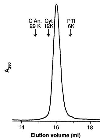
Fig. 8. Size exclusion chromatography indicating that Felix is a monomer under non-denaturing conditions. Felix S-S, at an initial concentration of 0.2 mg/ml, was chromatographed on a prepacked Superose-12 gel filtration column (Pharmacia) in 50 mM sodium phosphate, pH 7.6, 100 mM NaCl. Molecular size markers are carbonic anhydrase (C An), cytochrome c (Cyt), and bovine pancreatic trypsin inhibitor (PTI).
