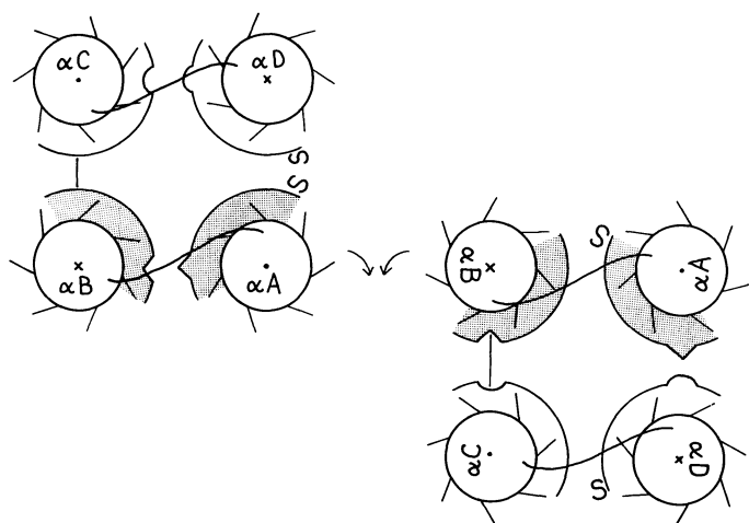
Fig. 4. The transformation between a left-turning and a right-turning helix bundle topology, with the \alpha A - \alpha B helix pair as a reference. Helices are viewed end-on, with a central dot for one coming up out of the page and an X for one going away. Some of the pinwheeling C\alpha - C\beta vectors are indicated. The hydrophobic half of each helix surface (stippled) contains two possible sites for contact with another helix. On the left, helices \alpha A and \alpha B interact with one pair of contacts (shown as triangles), leaving the other pair of contacts (shown smooth) available on their top surface for interacting with helices C and D; this produces a left-turning bundle topology. On the right, the two reference helices have rotated inward like meshed gears, bringing the smooth pair of contacts together and now leaving an open hydrophobic face on their lower surface against which helices C and D pack; this arrangement produces a right-turning topology.
